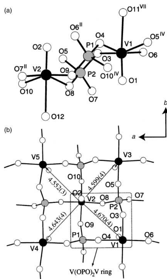
Fig. 2 Retracted chair conformation of [(\text{VO})_2(\text{PO}_4)_2]^- (a) and a section of a 4-connected net (b) in compound 1 . Water O atoms O11 and O12 and \text{Na}(\text{H}_2\text{O})_4 are omitted for clarity in (b), where \text{V} \cdots \text{V} distances (in Å) are indicated. Symmetry keys: II ( x + 1, y, z ), IV ( x, y - 1, z ), and VII ( x, y - 1, z - 1 ).
