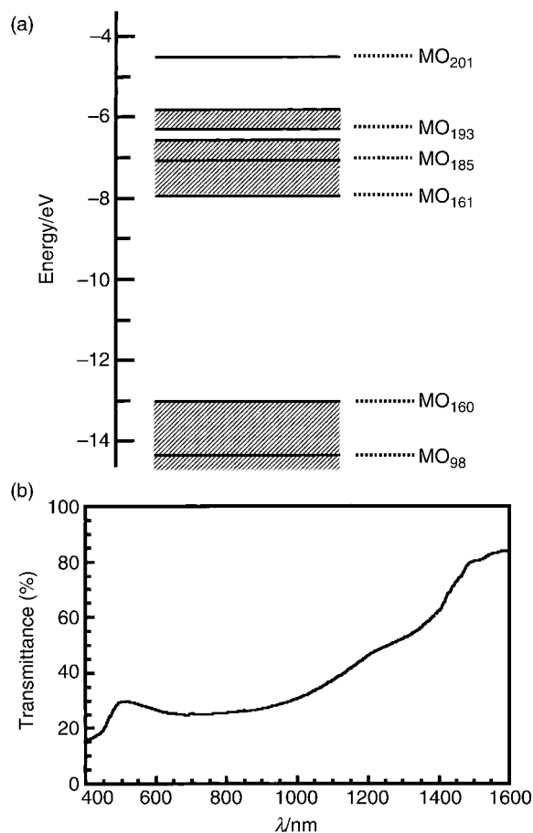
Fig. 7 Electronic energy-level scheme (a) for the fragment [\text{V}_8\text{P}_8\text{O}_{40}]^{4-} (with V^{\text{IV}}/V^{\text{V}} = 1/1 ) and diffuse reflectance spectrum (b) of compound 1 .
