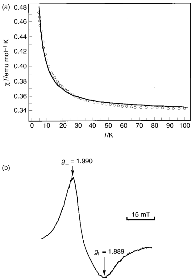
Fig. 4 (a) Plot of \chi T vs. T for compound 1 below 100 K. (b) The ESR spectrum of 1 at 4.2 K.
