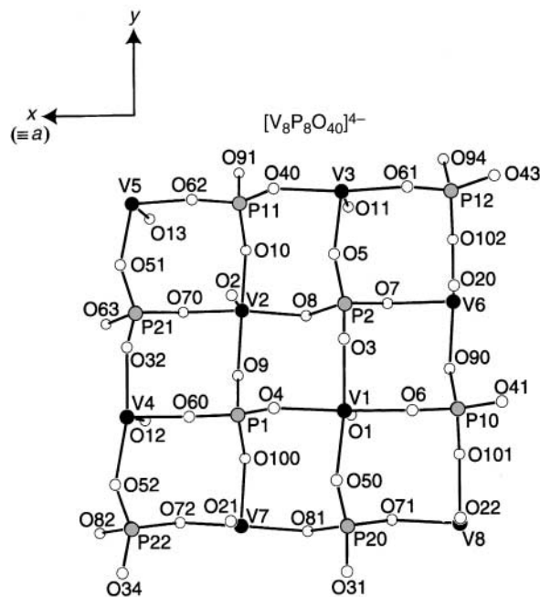
Fig. 6 The fragment [\text{V}_8\text{P}_8\text{O}_{40}]^{4-} (with V^{\text{IV}}/V^{\text{V}} = 1/1 ) and reference axes used for the EH calculation. The contribution of \text{Na}^+ cations and water molecules in the interlayer was neglected.
